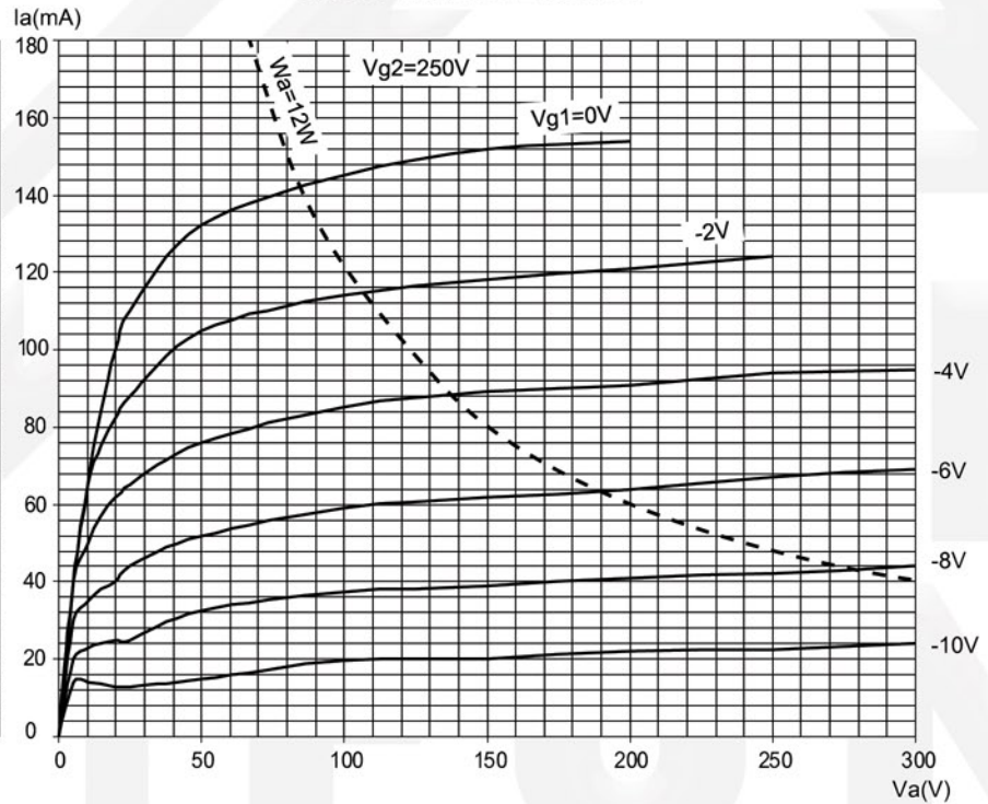
PLATE CHARACTERISTICS
